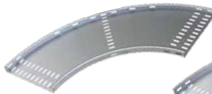
INSIDE RETURN FLANGE ELBOW HORIZONTAL - EHR
