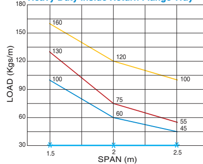
Extra Heavy Duty Inside Return Flange Tray
