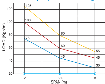
Double Extra Heavy Duty Inside Return Flange Tray
