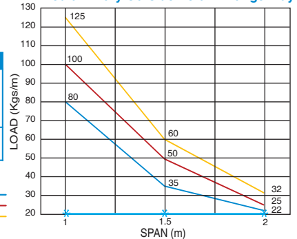
Heavy Duty Outside Return Flange Tray
